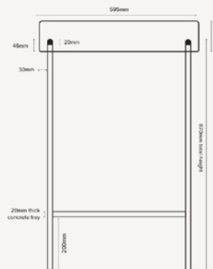
SECTION VIEW
