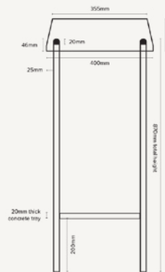
SECTION VIEW
