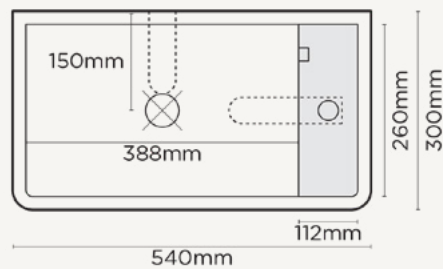
PLAN VIEW
