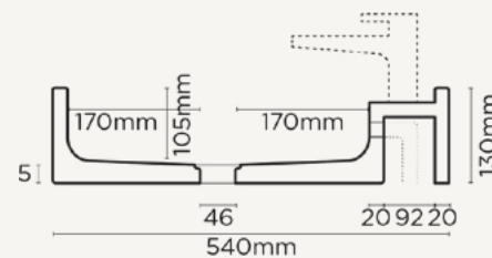
SECTION VIEW
