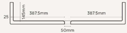
SECTION VIEW
