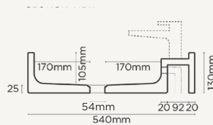
SECTION VIEW
