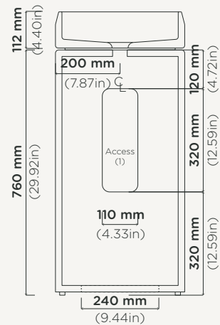
Section View Plumbing Access (2)
